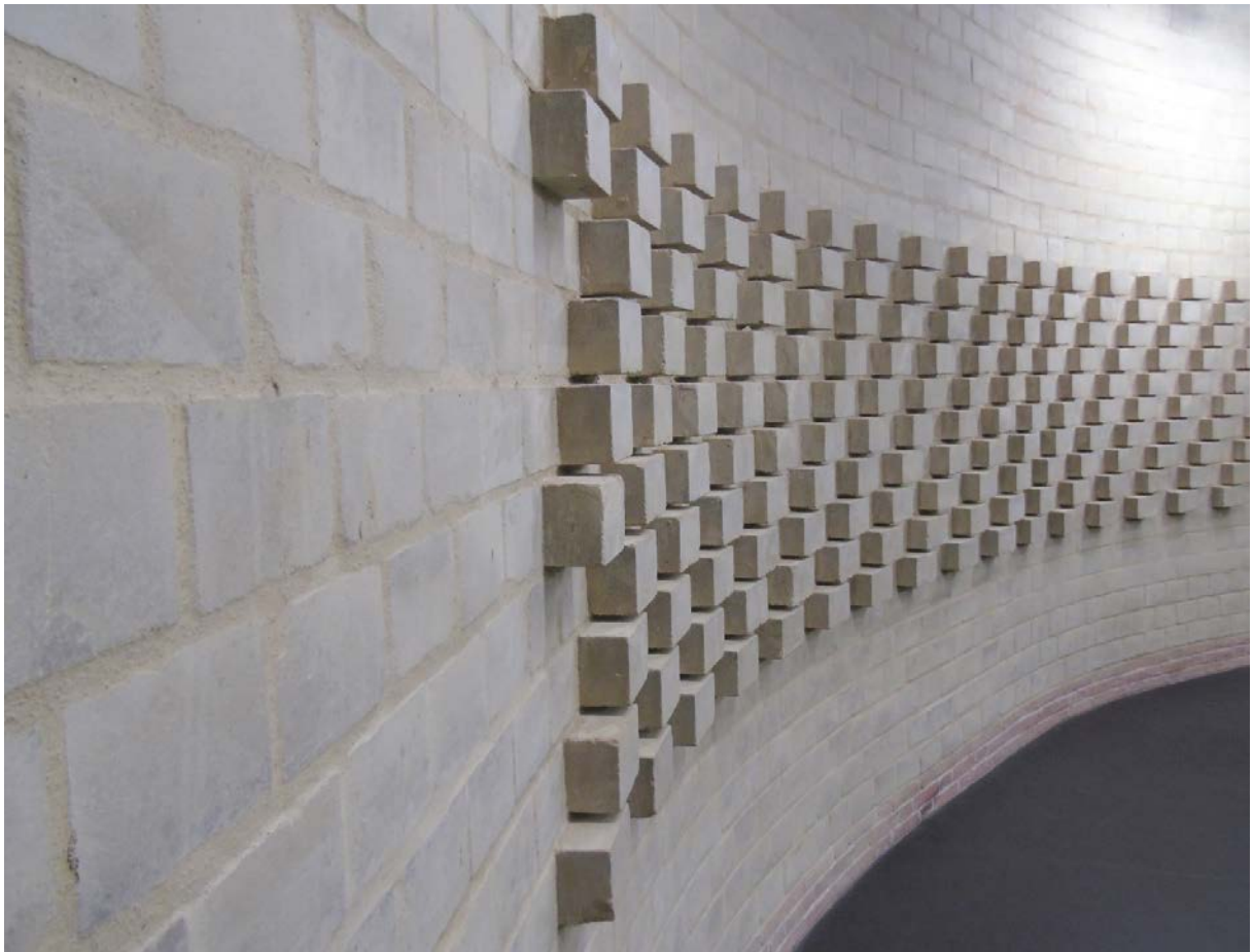
Compressed earth brick wall in Cornebarrieu, France (Photo credit: Daria Ardant)
