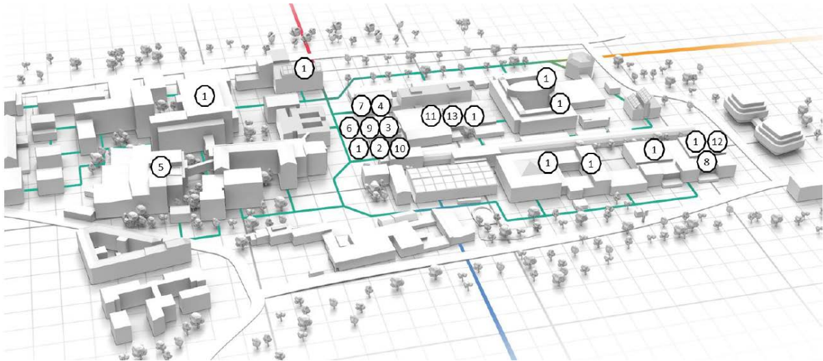
Figure 2: Completed infrastructure of the FED system, buildings that 'only' consume are visible, but not listed.
