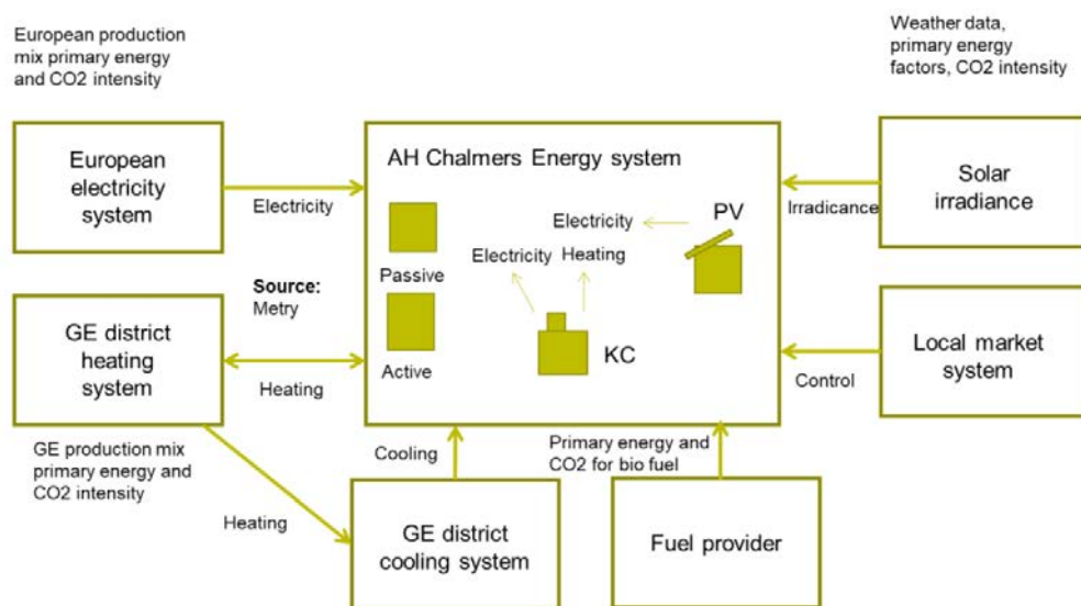
Figure 1: conceptual diagram of the energy flows between the external system and the FED system. (GE = Gothenburg Energi, the local energy supplier)
