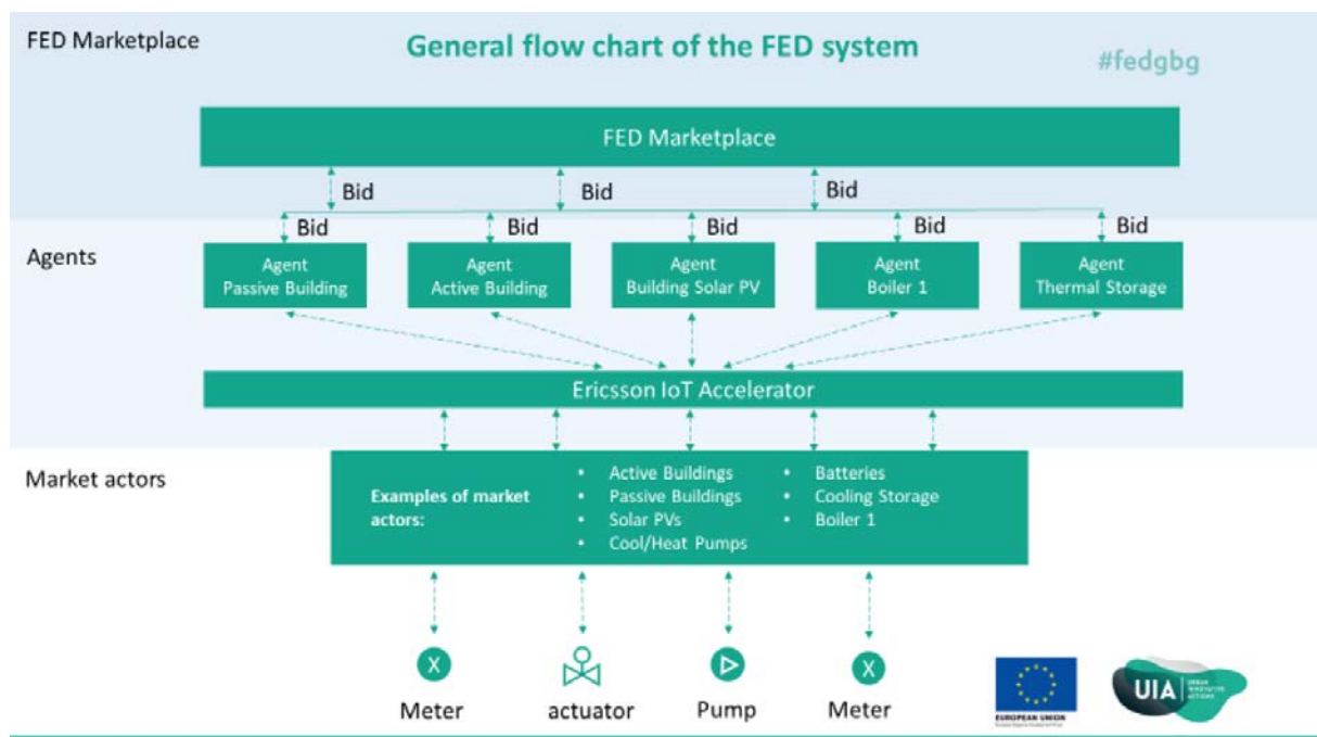
Figure 4: market solving in the FED
